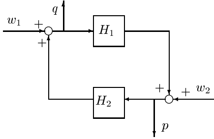
Figure 1: Internal stability
